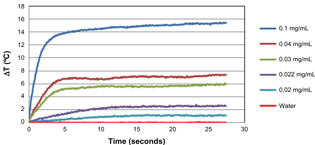
Figure 3 Temperature elevation as a function of irradiation time with the 663 nm laser for different concentrations of gold nanorods in aqueous solution. Note: The graph reaches a plateau after approximately 5 seconds.
