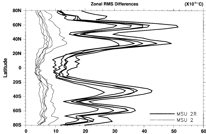
FIG. 12. Zonal means of the rms anomaly differences ( \times 10^{-2}^{\circ}\text{C} ) between different satellites for five overlap periods for MSU 2R (heavy lines) and MSU 2. The data were kindly provided by J. Christy.
