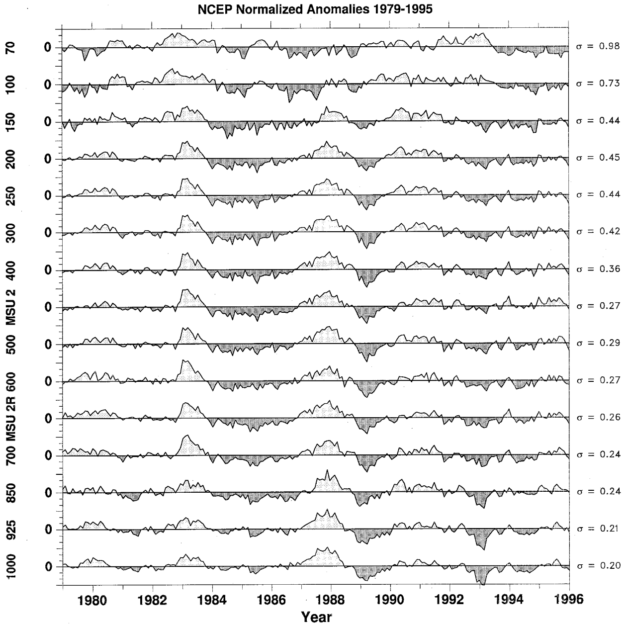
FIG. 9. Normalized tropical ( 20^{\circ}\text{S} – 20^{\circ}\text{N} ) temperature anomalies relative to the 1979–95 means of NCEP reanalyzed temperatures at pressure levels from 1000 to 70 mb. The standard deviations ( ^{\circ}\text{C} ) of the monthly anomalies are given on the right axis, and the tick marks on the left axis are every 3\sigma . The observed MSU 2R and MSU channel 2 normalized anomalies are also provided near the pressure levels of the peaks in their respective weighting functions. Negative anomalies are given by the darker shading.
