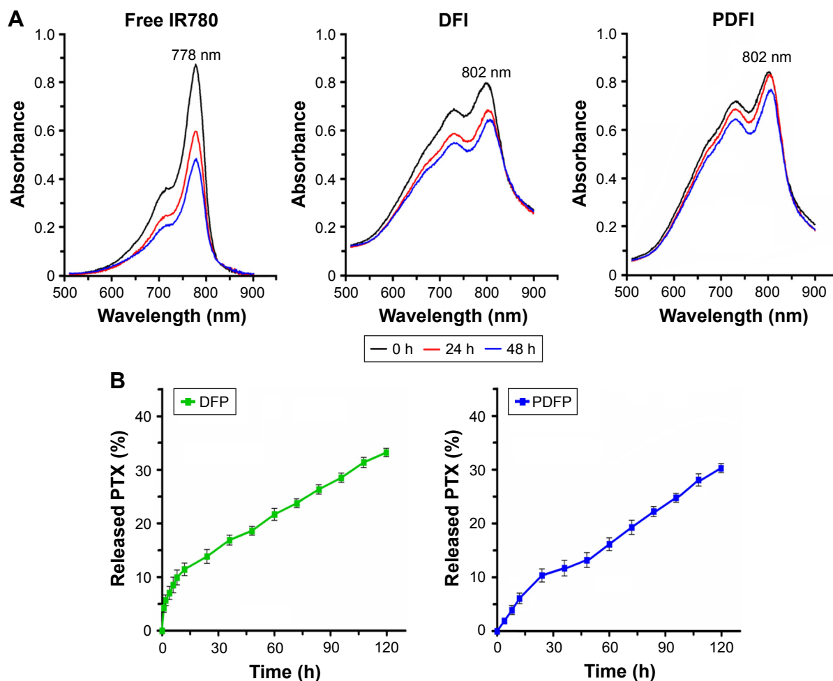
Figure 2 The ultraviolet-visible spectra of free IR780, DFI nanocores and PDFI nanoparticles in water at IR780 concentration of 5 \mu\text{g/mL} (A), and the in vitro releases of PTX from DFP nanocores and PDFP nanoparticles in phosphate buffer saline solution at pH 7.4 (B).
