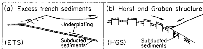
Figure 15 Two trench morphologies. (a) Excess trench sediments. Sediments are scraped off on subduction and form an accretionary prism. (b) Horst-and-graben structure. A well-developed horst-and-graben structure provides a mechanism to carry down the sediments (after Ruff 1985).
