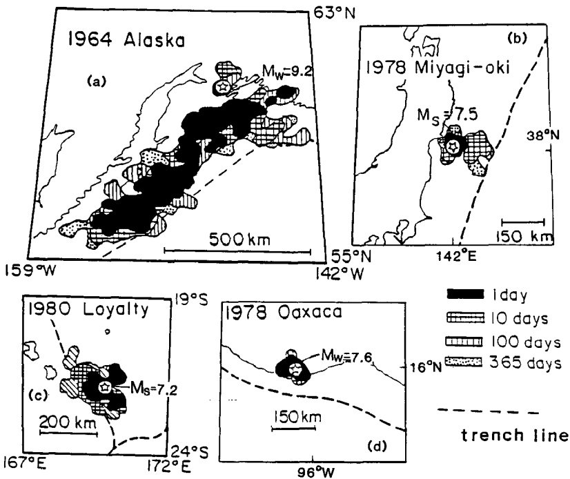
Figure 12 The aftershock areas determined at four different times: 1 day, 10 days, 100 days, and 1 yr (slightly modified from Tajima & Kanamori 1985b).
