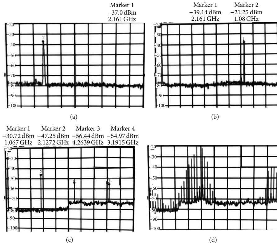
FIGURE 13: Spectrum analyzer display of Oscillator-type active antenna (a) periodic mode, (b) period-doubled mode, (c) period-four mode, and (d) chaotic mode.
