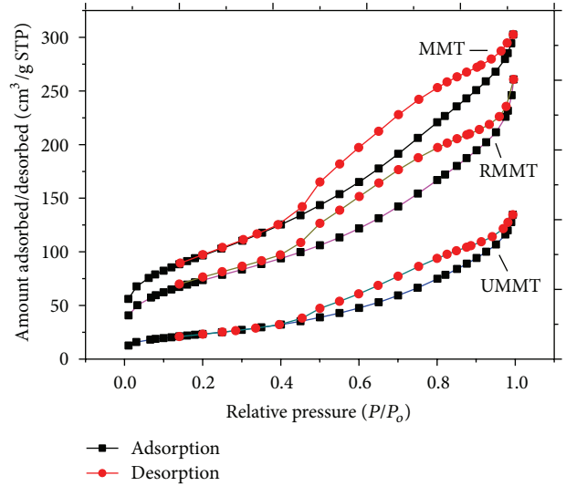
FIGURE 7: \text{N}_2 adsorption-desorption isotherms of MMT, UMMT, and RMMT.
