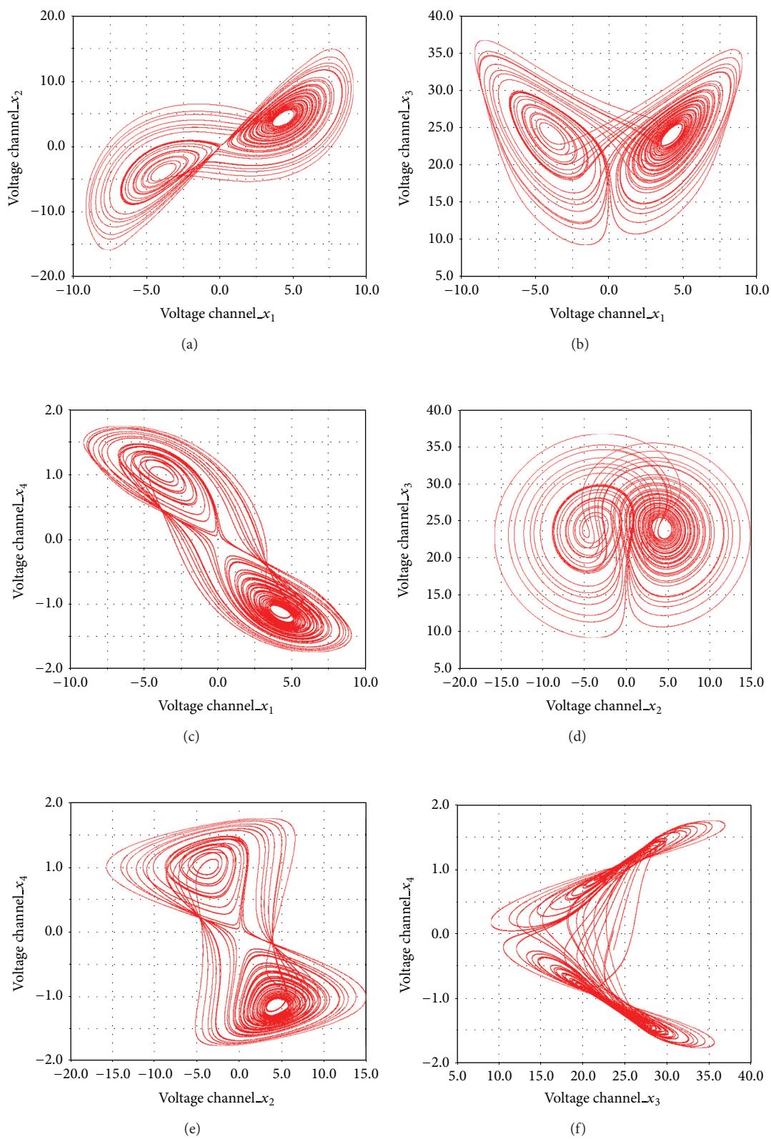
FIGURE 9: Oscilloscope graphics for voltage signals outputs of the four-dimensional Lorenz-Stenflo system: (a) V_{x_1} - V_{x_2} , (b) V_{x_1} - V_{x_3} , (c) V_{x_1} - V_{x_4} , (d) V_{x_2} - V_{x_3} , (e) V_{x_2} - V_{x_4} , and (f) V_{x_3} - V_{x_4} .
