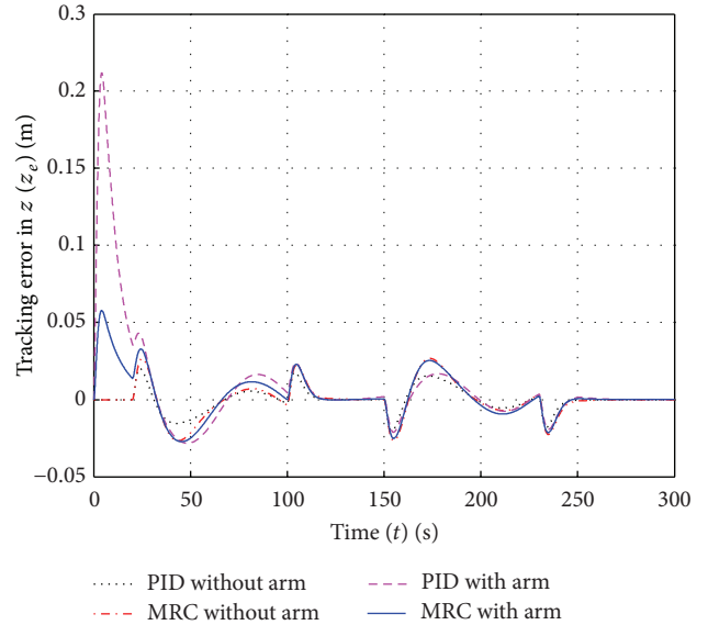
FIGURE 8: Tracking errors in z position for a given 3D trajectory.
