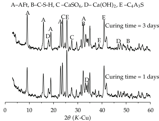
Figure 3: XRD pattern of SCM after hydration for 1 and 3 days.
