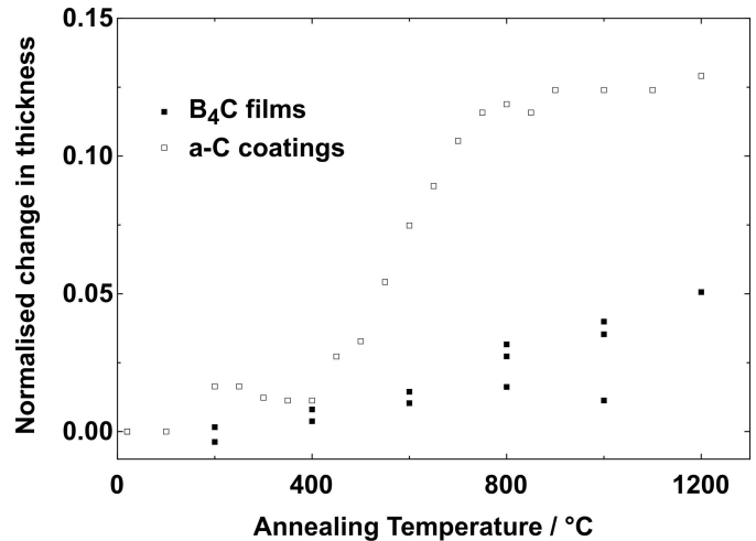
Figure 6 Variation in layer thickness of annealed boron carbide and carbon coatings.
