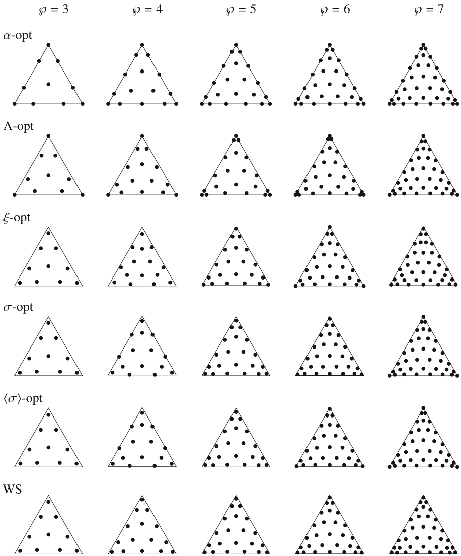
Fig. 6 Plots of \alpha -optimised, \Lambda -optimal, \xi -optimal, \sigma -optimal, \langle\sigma\rangle -optimal, and WS rules on an equilateral triangle for various orders. The location of these points are tabulated, along with the associated quadrature weights, in Appendix. They are also available in Online Resource 1
