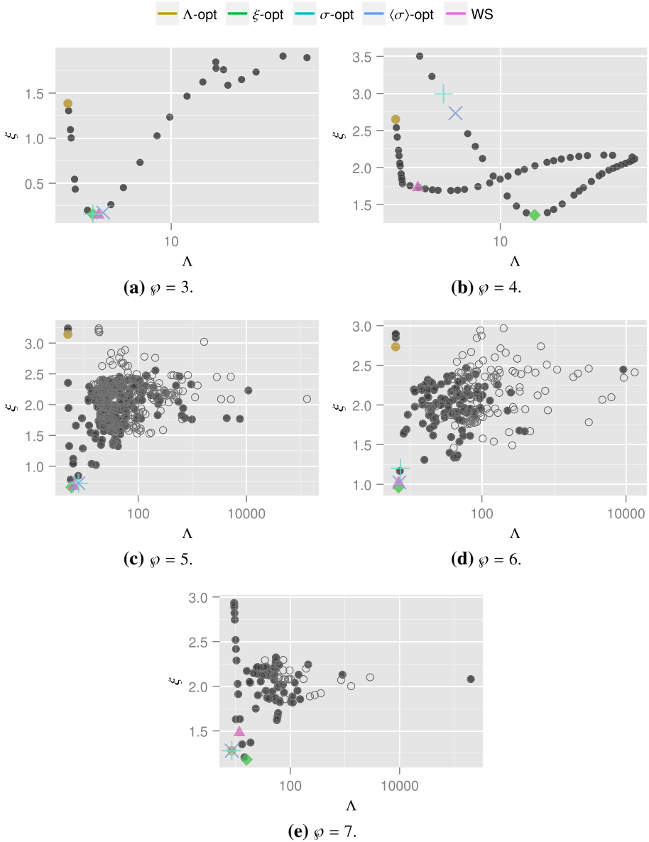
Fig. 4 Semi-log plots of the Lebesgue constant, \Lambda , against truncation error, \xi , for all point sets. Rules which do not make it to t = 100 are indicated by hollow markers. \Lambda -optimal points are denoted by a gold circle, \xi -optimal by a green diamond, \sigma -optimal by a teal '+', \langle\sigma\rangle -optimal by a blue 'x' and WS by a pink triangle (Color figure online)
