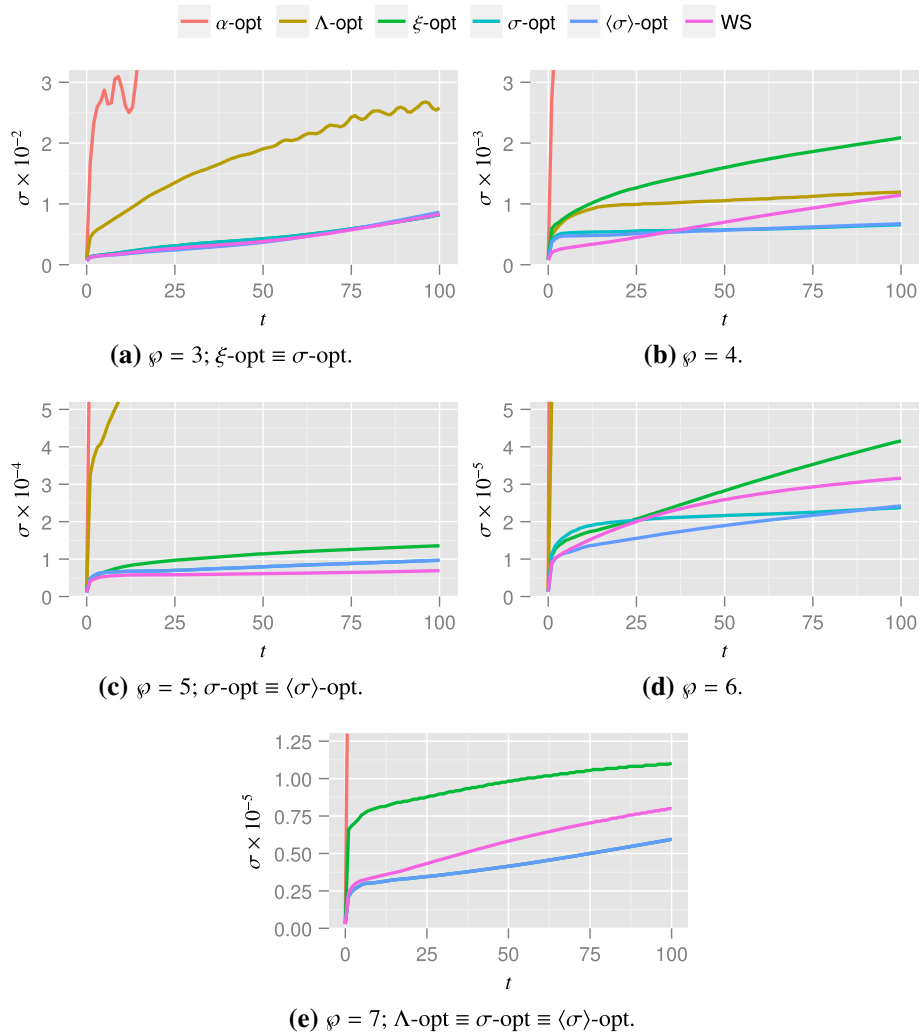
Fig. 5 L^2 error against time for the \alpha -optimised, \Lambda -optimal, \xi -optimal, \sigma -optimal, \langle\sigma\rangle -optimal and WS points. Quantitative details of the L^2 error at t = 100 for all point sets shown can be found in Table 4
