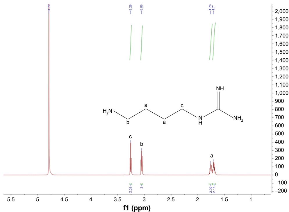
Figure S1 1 H nuclear magnetic resonance spectroscopy of agmatine sulfate.
