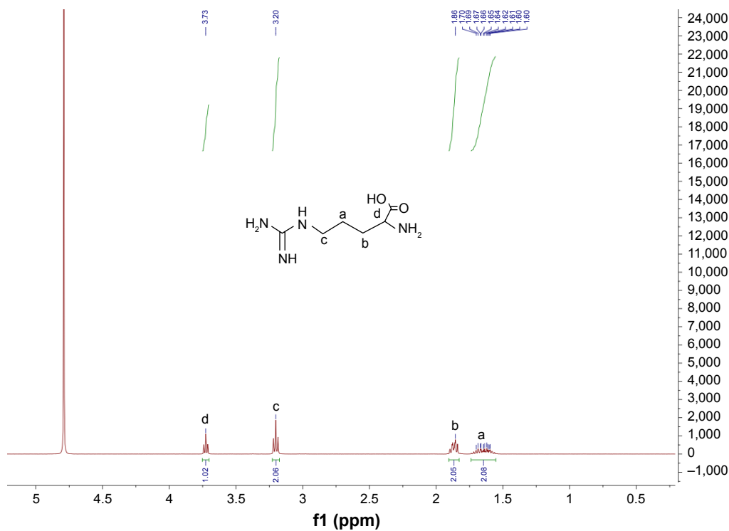
Figure S4 1 H nuclear magnetic resonance spectroscopy (NMR) of L-arginine (Arg).
