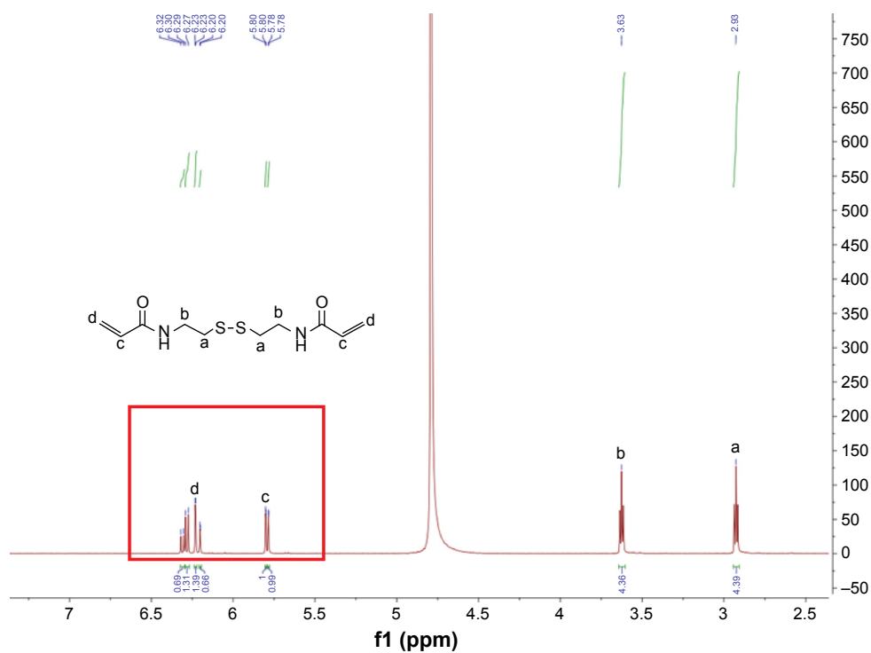
Figure S2 1 H nuclear magnetic resonance spectroscopy of N,N' -cystamine bisacrylamide.
