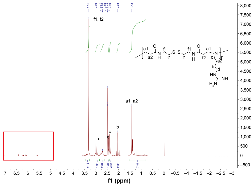
Figure S3 1 H nuclear magnetic resonance spectroscopy (NMR) of Agm-CBA.
