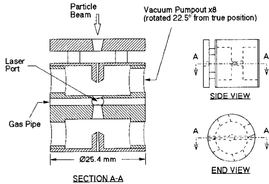
Figure 3: Plasma Chamber
