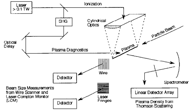
Figure 1: Outline of Plasma Lens Experimental Setup
