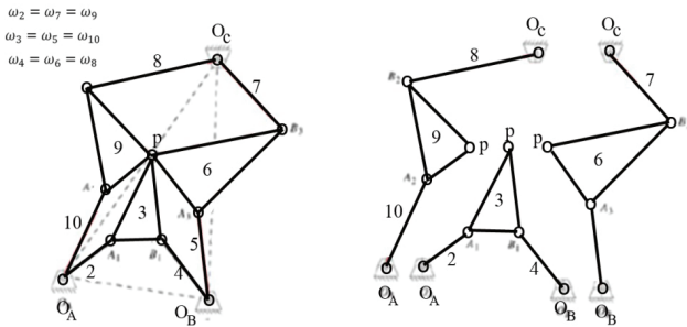
Figure 7. Procedure of drawing cognates of a mechanism
