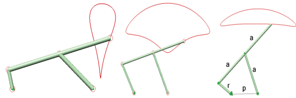
Figure 2. different shapes of coupler curves generated by the same type of mechanism
