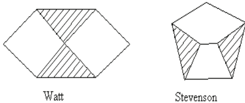
Figure 8. Two basic kinematic chains belonging to the six-bar 1 degree of freedom class of mechanisms
