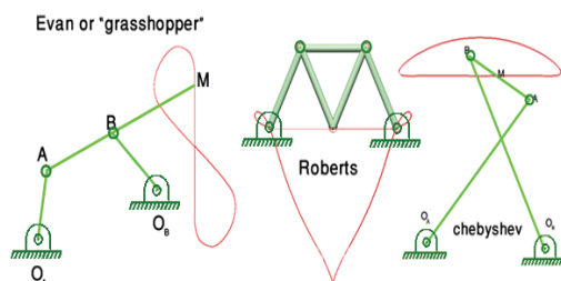
Figure 1. Three known straight line generating mechanisms
