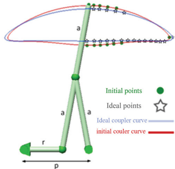
Figure 5. Initial versus Ideal path
