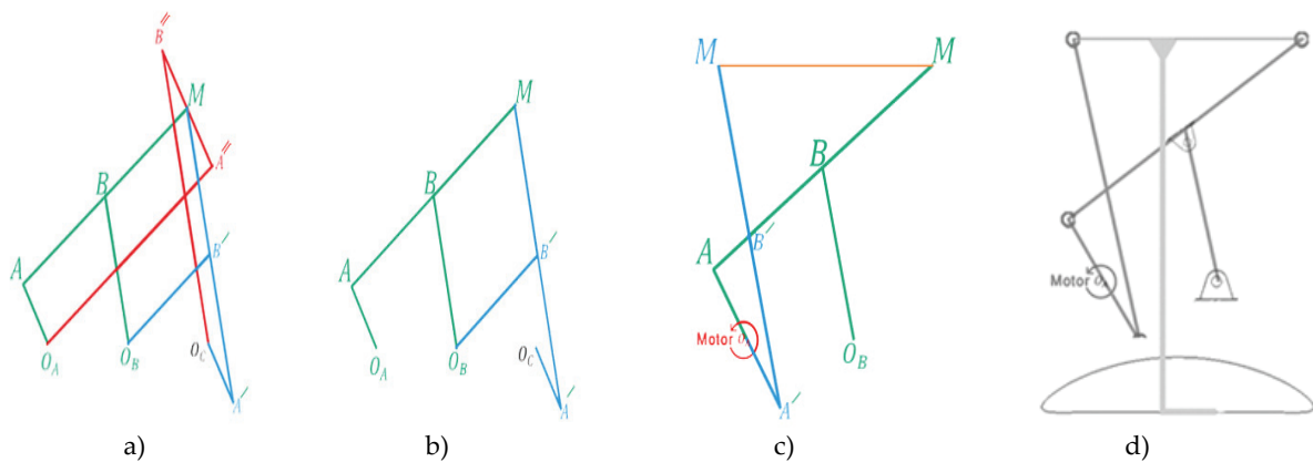
Figure 10. Different stages of establishing the Watt's six-bar linkage with leg connected to straight and parallel moving link
