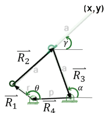
Figure 3. Linkage notation
