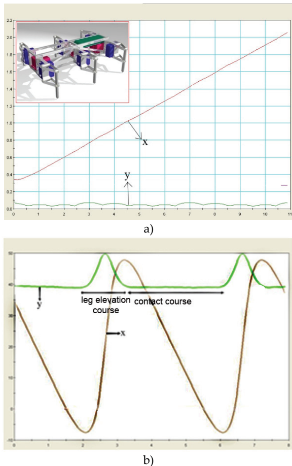
Figure 11. [11] a) Center of mass position of a hexapod versus time b) Position of each point on the leg versus time
