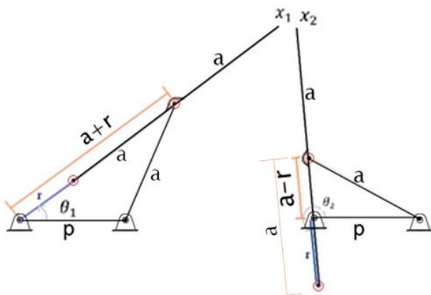
Figure 4. Critical points and angles
