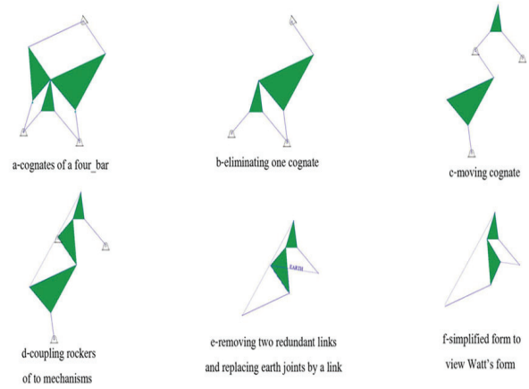
Figure 9. Procedure of obtaining Watt six-bar linkage from optimal four-bar
