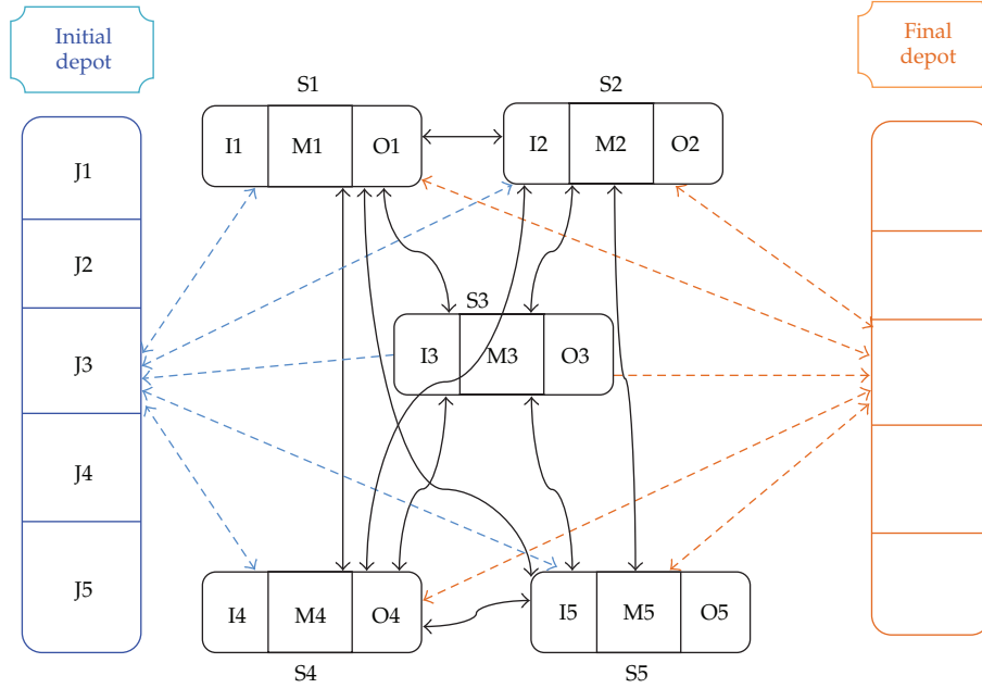
Figure 2: Problem graph.
