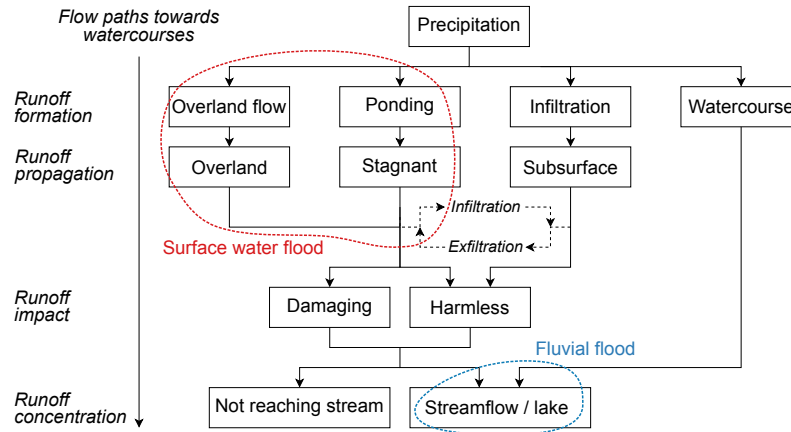
Figure 1. Interrelation of hydrological processes that may lead to a surface water flood (red ring) and/or a fluvial flood (blue ring).
