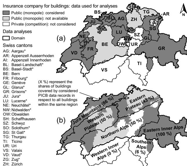
Figure 3. Overview of the compiled data set D1 (see Table 3). (a) Cantons with and without a PICB and an indication of which PICBs provided data. The latter are additionally marked with an asterisk (*) in the legend. (b) Natural landscape units based on Grosjean (1975), which are used to analyze the data on a regional scale. As almost no buildings are insured by PICBs within the Western Inner Alps or the Southern Alps, these two regions are excluded from the data analyses, as indicated by the domain.
