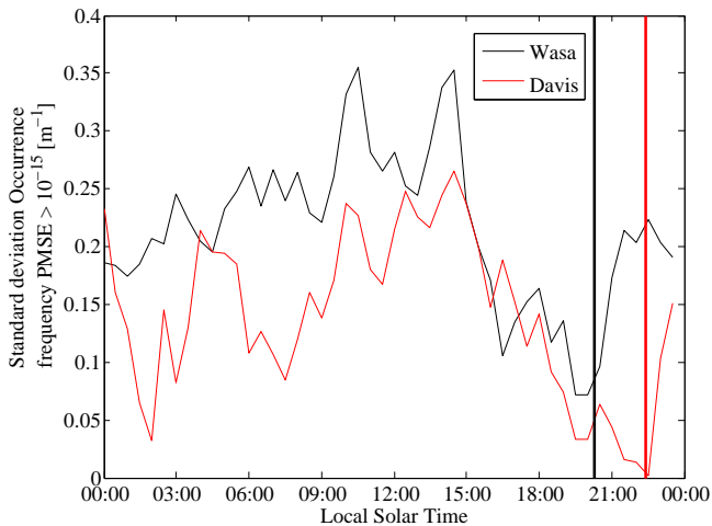
Fig. 5. The standard deviation of the occurrence frequency in the altitude interval 82–88 km as a function of local solar time. Data from MARA Wasa are shown with a black line, data from Davis with a red line. Thick vertical bars indicate 19 magnetic local time at Wasa (black) and at Davis (red).
