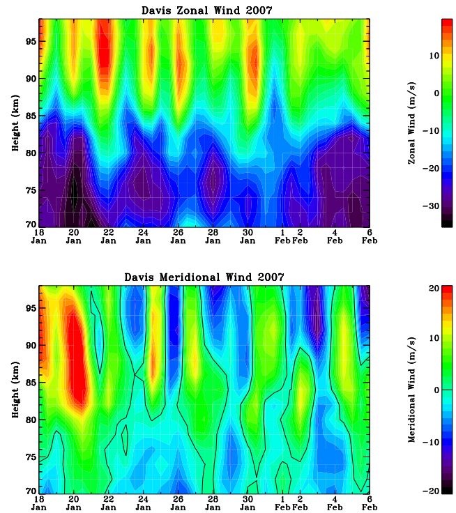
Fig. 3. Davis MF radar wind data, running average over 1 day. The top panel shows the zonal wind and the bottom panel the meridional wind [ \text{m s}^{-1} ], as a function of date (x-axis) and height (y-axis).
