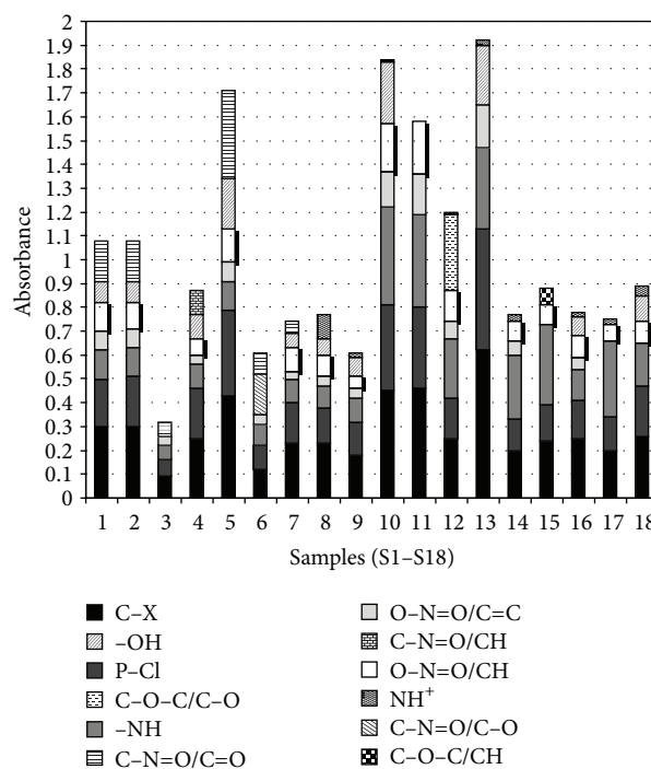
FIGURE 2: The number, type, and absorbance value of the main functional groups in NSOMs.
