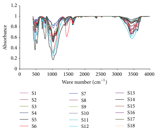
FIGURE 1: Infrared spectra of eighteen soil samples (S1 to S18).
