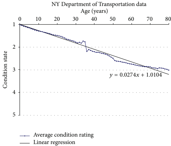
FIGURE 8: New York Department of Transportation condition state data.
