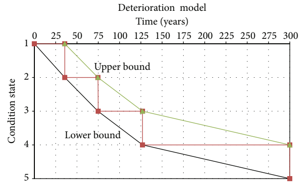
FIGURE 11: Markov chain deterioration model.
