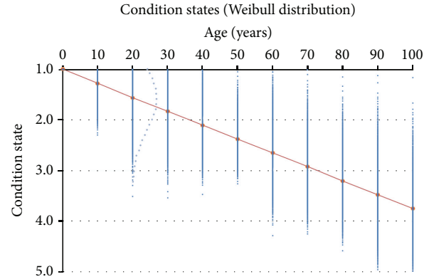
FIGURE 9: Synthetic condition state values.
