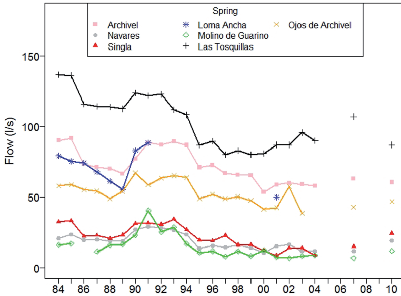
Figure 4: Official values of the mean volume of flow (l/s) of some of the springs of the Revolvedores-Serrata unit from 1984 to 2010. Source: adapted from Cabezas 2010.
