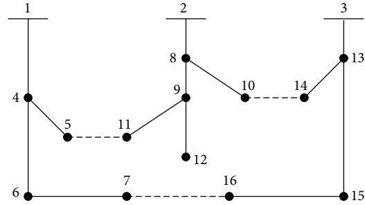
FIGURE 3: IEEE distribution system diagram with 16 feeders.
