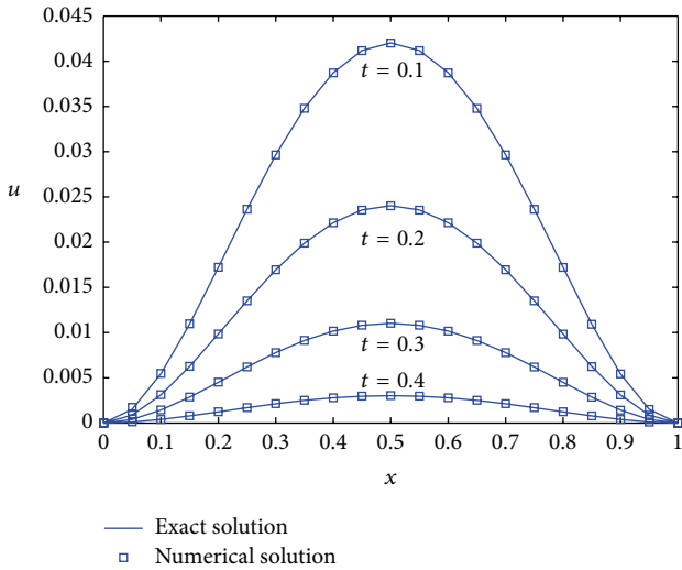
FIGURE 1: Numerical solution and exact solution for Example 1.
