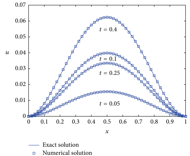
FIGURE 3: Numerical solution and exact solution for Example 3.
