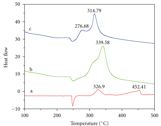
FIGURE 1: DSC thermal decomposition curves of AP. (a) pure AP; (b) nano-CuO simple mixed with AP; (c) nano-CuO/AP composite.
