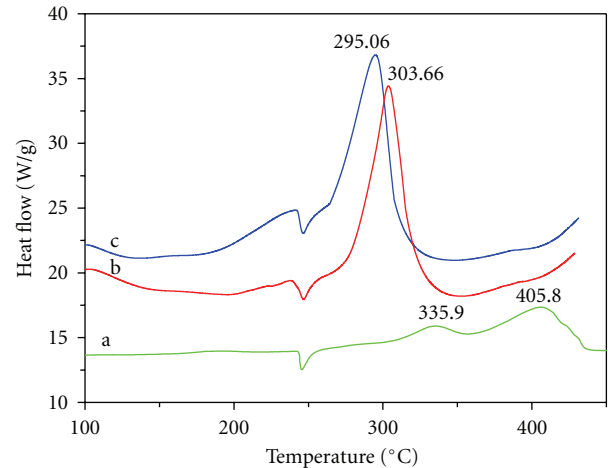
FIGURE 2: DSC curves of AP/HTPB propellant kneaded 4 hours. (a) Blank sample (b) Propellant with nano-CuO (Area 1); (c) Propellant with nano-CuO/AP (Area III).
