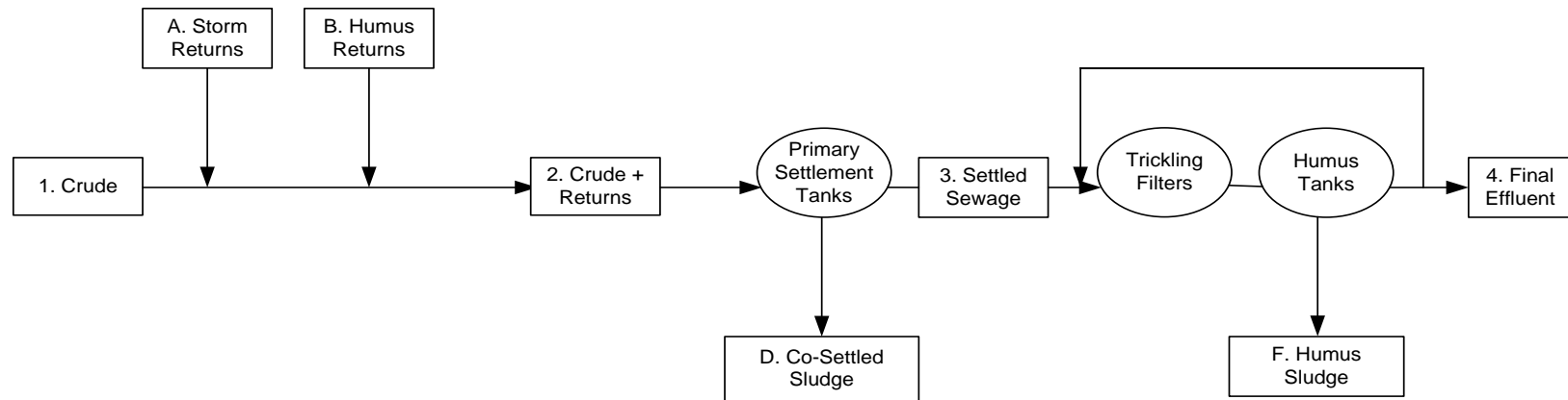
Figure 1. A - the concentrations (mg L -1 or µg L -1 ) of measured parameters in the wastewater at site 1. B - the site process flow diagram. Circles represent the unit treatment processes while the numbered or lettered boxes indicate the sampling points.
