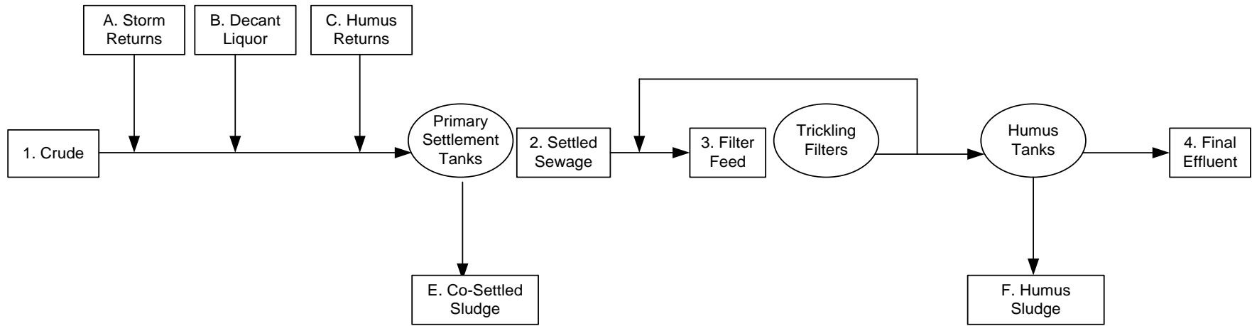
Figure 2. A - the concentrations (mg L -1 or µg L -1 ) of measured parameters in the wastewater at site 2. B - the site process flow diagram. Circles represent the unit treatment processes while the numbered or lettered boxes indicate the sampling points.
