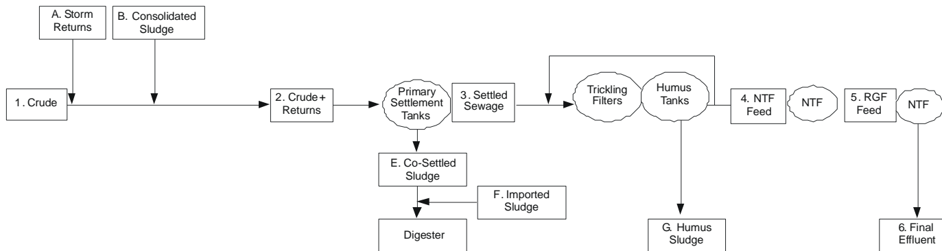
Figure 6. A - the concentrations (mg L -1 or µg L -1 ) of measured parameters in the wastewater at site 6. B - the site process flow diagram. Circles represent the unit treatment processes while the numbered or lettered boxes indicate the sampling points.
