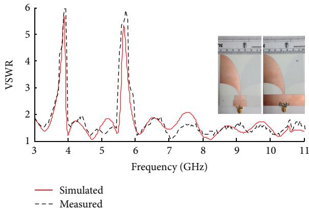
FIGURE 7: Simulated and measured VSWS of the proposed AVA.
