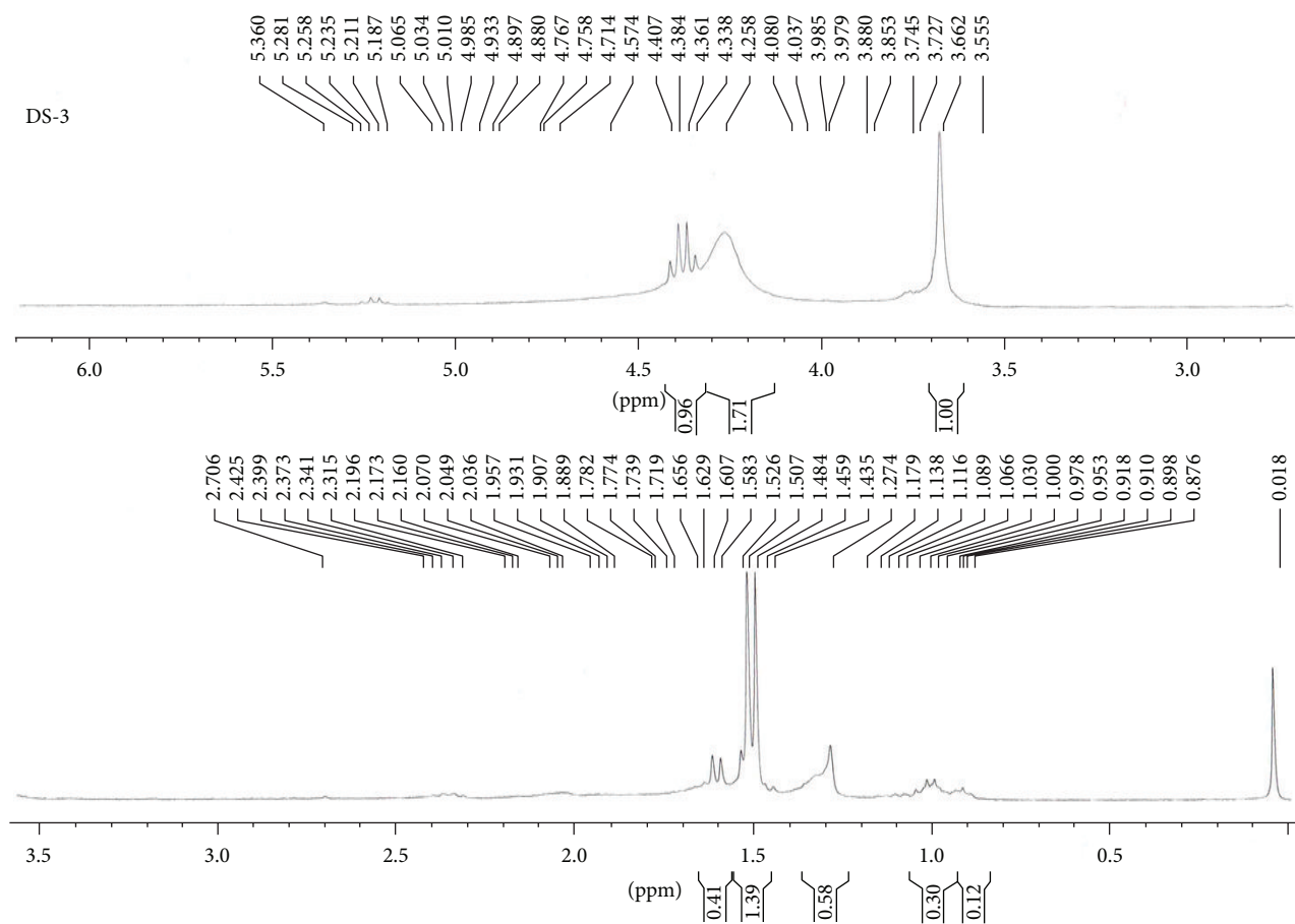
FIGURE 4: ^1\text{H} NMR spectrum of biosurfactant produced by Lactobacillus casei MRTL3.
