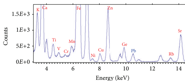
FIGURE 2: TXRF spectrum of a moss sample from Tollocan sampling site (6) at the Metropolitan Zone of the Valley of Toluca.
