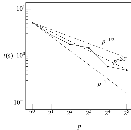
Fig. 6. Execution time for a Cray-X1E as a function of the number of images. The matrix size is n = 5000 and the block size is nb = 50 . Perfect scaling corresponds to the dashed line marked p^{-1} . Our code scales approximately as p^{-2/3} .
