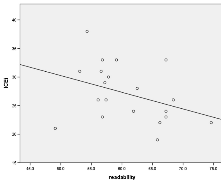
Figure 1 Correlation of readability and overall score.
