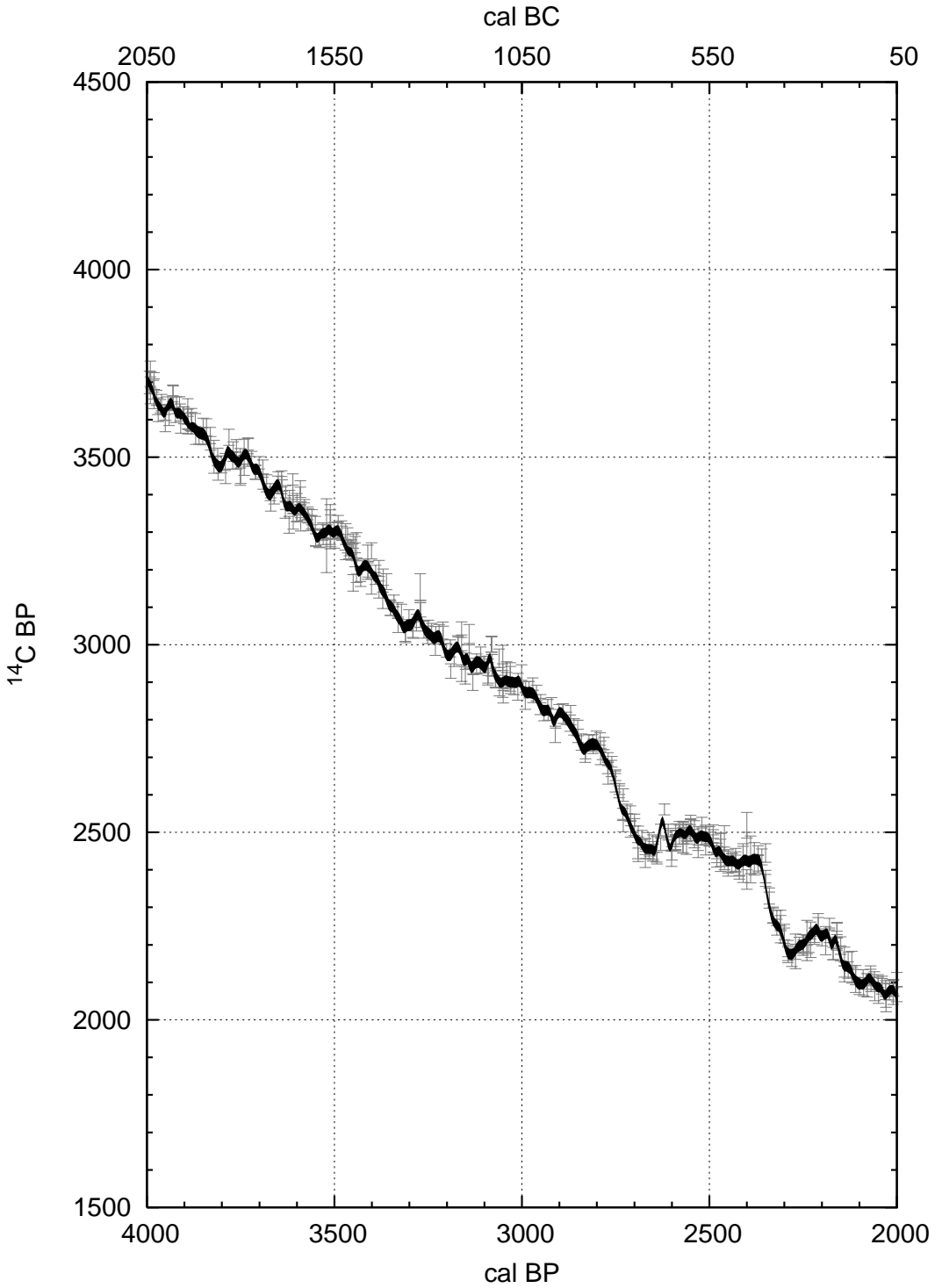
Figure A12 The IntCal04 terrestrial calibration curve (1-standard deviation envelope) and data with 1-standard deviation error bars in 14 C increased by the laboratory error multipliers described in the text. The uncertainty in the calendar ages is not shown, but is taken into account in the random walk model.
