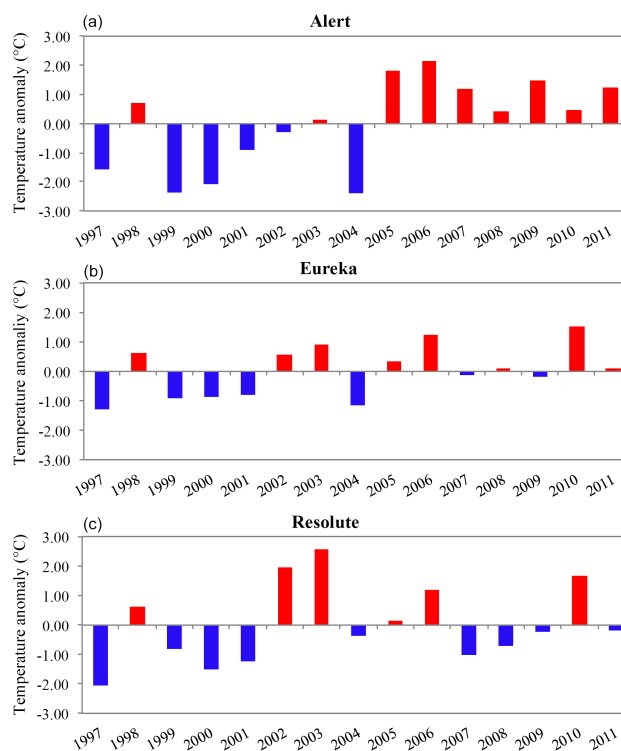
Figure 3. Air temperature anomalies for (a) Alert, (b) Eureka, and (c) Resolute relative to the 1997–2011 mean annual temperature.
