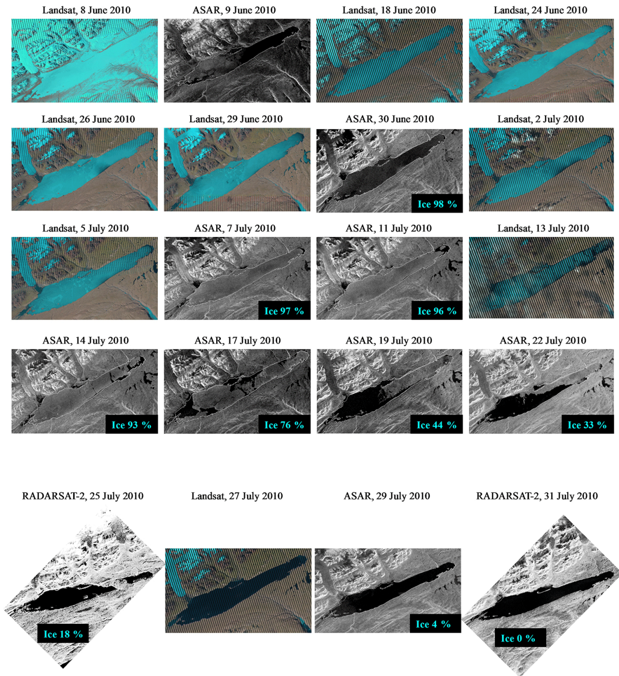
Figure 9. Time series of combined satellite observations (Landsat, ASAR, and RADARSAT-2) for Lake Hazen during the break-up period of 2010. RADARSAT-2 Data and Products © MacDonald, Dettwiler and Associates Ltd., 2010, all rights reserved. RADARSAT is an official trademark of the Canadian Space Agency. Ice fractions for available SAR images are also shown. No ice fractions are shown for Landsat observations as image segmentation was only performed on SAR imagery.
