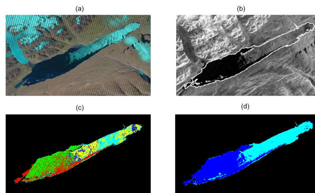
Figure 2. SAR-image segmentation processing steps: (a) Landsat image of Lake Hazen, 19 July 2010; (b) original ASAR image of Lake Hazen acquired on 19 July 2010; (c) K -means classified image (five clusters); (d) two-class map of ice (light blue) and open water (dark blue). The white line in the original SAR image represents the lake polygon that was used for defining the ROIs covering the lake.
