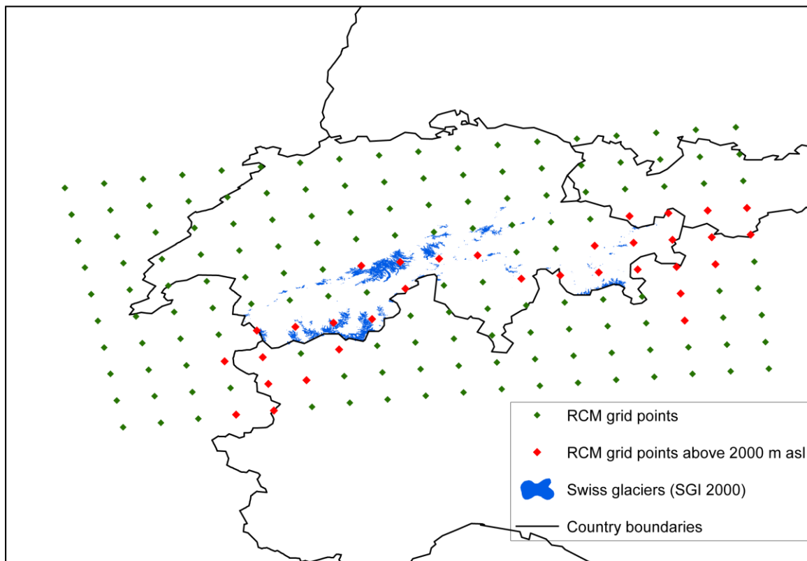
Figure S2: The RCM grid points used in this study.
