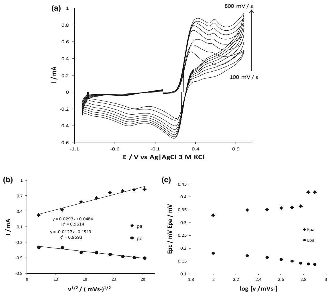
Fig. 10 Cyclic voltammograms of the Pt/NiNP modified electrode at different scan rates in 0.005 M [\text{Fe}(\text{CN})_6]^{3-}/[\text{Fe}(\text{CN})_6]^{4-} 0.2 M NaOH solution (a), scan rates from 100 to 800 mV/s. Dependence of
