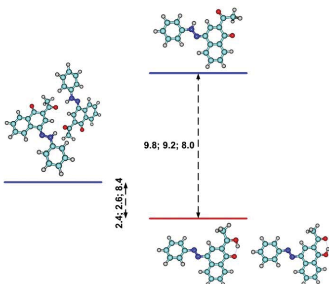
Fig. 8. Relative stability (HF/6–31G**) of the tautomers of 4 . The values of the relative energy, relative energy + ZPE correction and ΔΔG are given in kcal/mol units.
