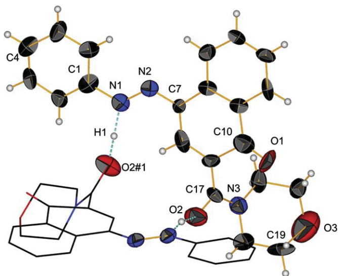
Fig. 6. View of molecular structure of 3b , 50% of probability, H-bond are drawn in dashed blue, solvent molecules and some hydrogen atoms are omitted for clarity, #1: 1– x , y , 0.5– z . (For interpretation of the references to colour in this figure legend, the reader is referred to the web version of this article.)
