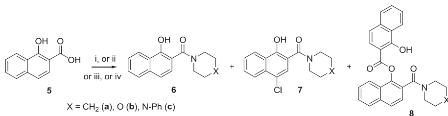
Scheme 2. i) piperidine, EDCl, HOBT, CH 2 Cl 2 , rt; ii) 1. SOCl 2 , reflux; 2. piperidine, CH 2 Cl 2 , rt; iii) SOCl 2 (4 equiv), DMF, heptane, reflux, 4 h; 2. piperidine or morpholine, i -Pr 2 NEt, CH 2 Cl 2 , rt; iv) 1. SOCl 2 (2.5 equiv), DMF, heptane, reflux, 4 h; 2. piperidine or morpholine, i -Pr 2 NEt, CH 2 Cl 2 , rt.
