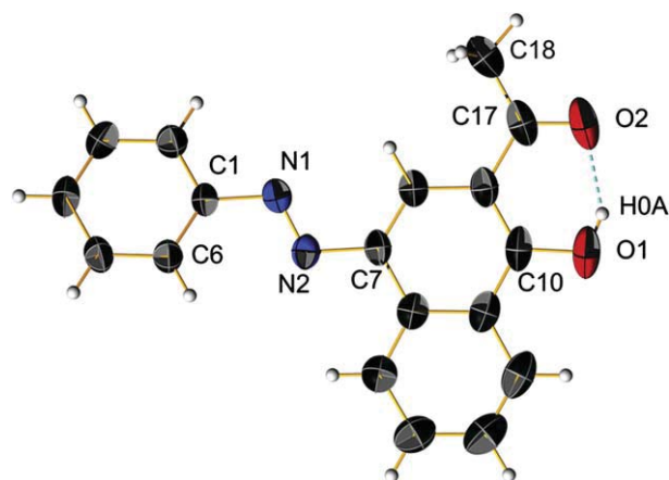
Fig. 9. View of the molecular structure of 4 , 30% of probability. H atoms are presented with spheres of arbitrary radii. H-bond is shown in dashed blue. (For interpretation of the references to colour in this figure legend, the reader is referred to the web version of this article.)
