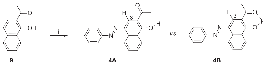
Scheme 4. i) PhNH 2 , conc. HCl, NaNO 2 , acetone–H 2 O, NaOH.
