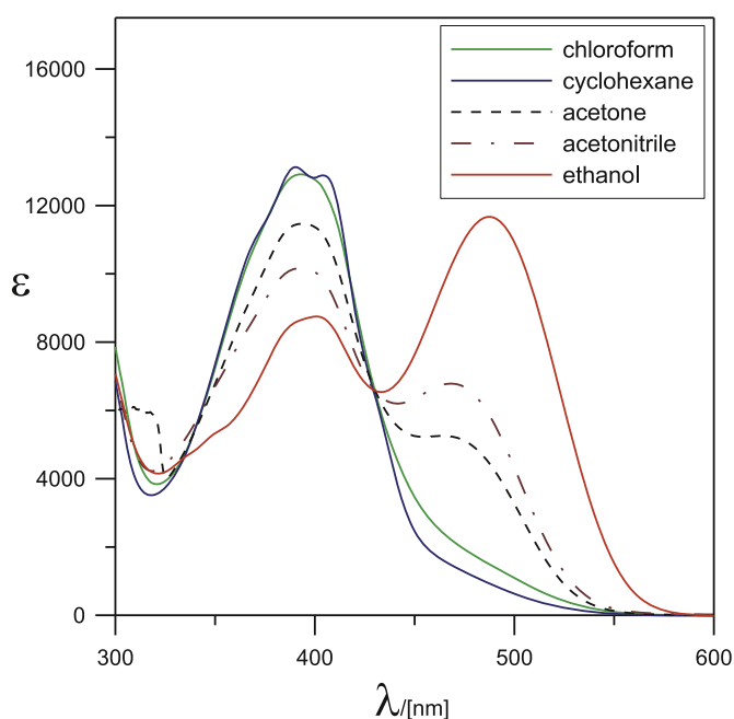
Fig. 2. Absorption spectra of 3a in various solvents.
