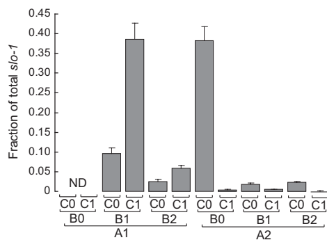
Fig. S3. Measured distribution of the 12 s/o-1 variants in wild type. Copy numbers of each s/o-1 splice variant were measured by CAE-qPCR, and the fraction of the total copy number is shown for each splice variant. Errors bars are 99% confidence intervals of the means. ND, not detectable.
