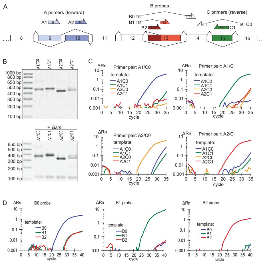
Fig. S1. CAEq-PCR method. (A) Schematic of the alternatively spliced region of slo-1 and primer and probe recognition sequences. (B) Qualitative analysis of PCR products for each A/C primer pair. The template was a cDNA library generated by RT with random hexamers and a slo-1 gene-specific primer from total adult worm RNA extracts. PCR products were digested with BsmI where indicated, yielding fragments of the expected size for slo-1 specific amplification. (C) The specificity of each A/C primer pair was assessed by real-time PCR analysis (SYBR green). Each panel depicts representative amplification curves for the indicated A/C primer pair. In each case, separate reactions were run with four plasmid templates carrying the indicated slo-1 splice variants (one match, three mismatches). \Delta R_n , relative fluorescence changes after baseline subtraction. (D) The specificity of each B probe was assessed by probe-hydrolysis (Taqman) qPCR with matched A/C primers. Each panel depicts representative amplification curves for the indicated probe. In each case, separate reactions were run with three plasmid templates carrying the indicated slo-1 splice variants (one probe match, two probe mismatches). \Delta R_n , relative fluorescence changes after baseline subtraction.
