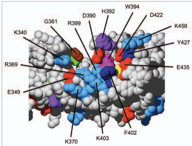
Figure 4. The highly conserved surface area in domain 8–10 of the ankyrin domain of petunia VAPYRIN. Close-up of the highly conserved region of petunia PAM1 as shown in Figure 3G. Amino acids were color-coded as in Figure 3 and their position in the amino acid sequence is indicated (compare with Sup. Fig. 1).
