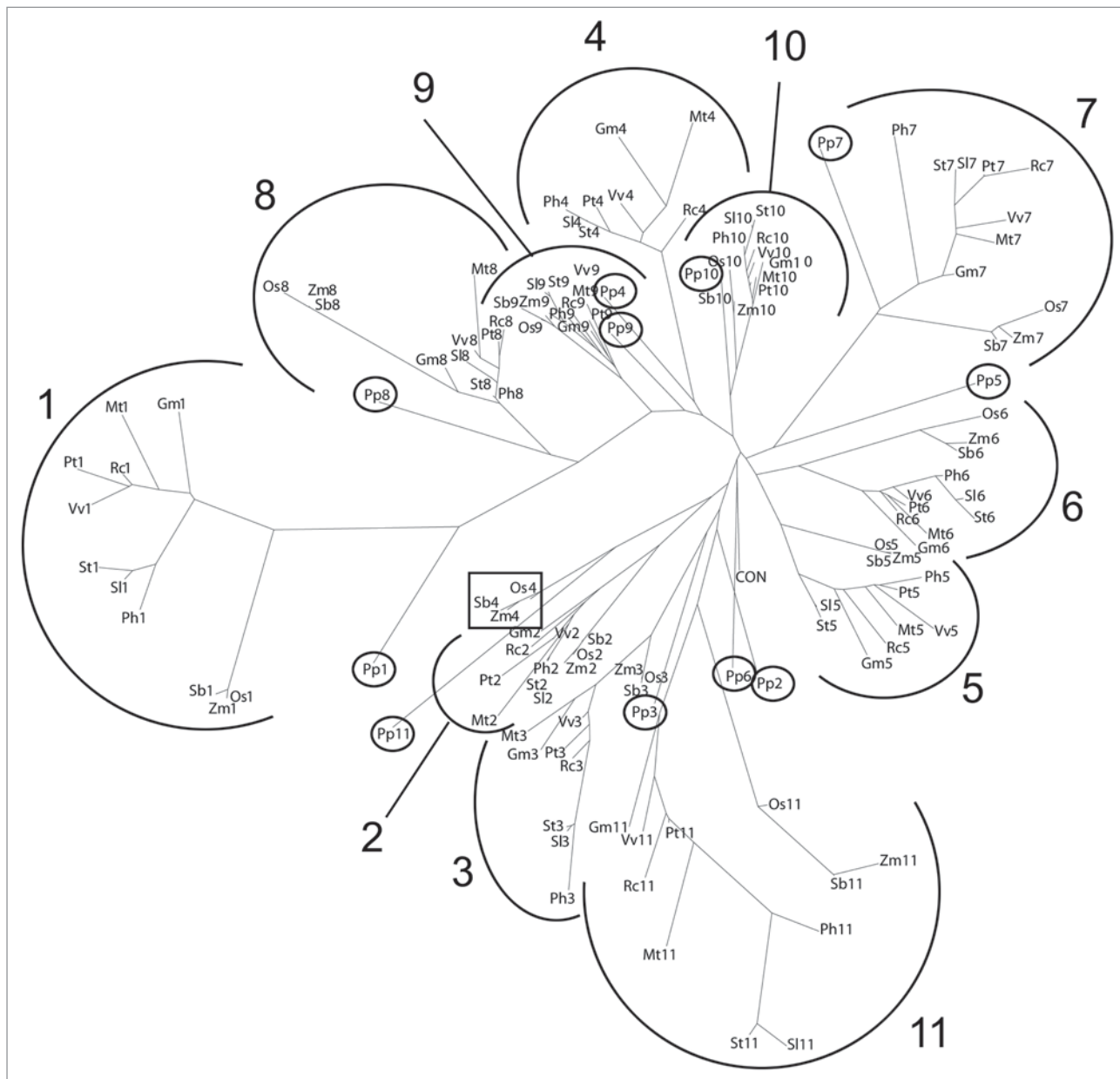
Figure 2. Phylogenetic analysis of the individual ankyrin repeats of VAPYRIN. Phylogenetic representation of an alignment of all the 11 repeats of the 12 VAPYRINs compared in Figure 1B and C . The repeats cluster according to their position within the domain, rather than to their origin (plant species). Numbers indicate the position of the repeats within the domain (compare with Fig. 1C ). P. patens repeats are highlighted (small circles) for clarity. The monocot repeat 4 sequences (boxed) are remote from the remaining repeat 4 sequences because of the grass loop (compare with Fig. 1C ).
