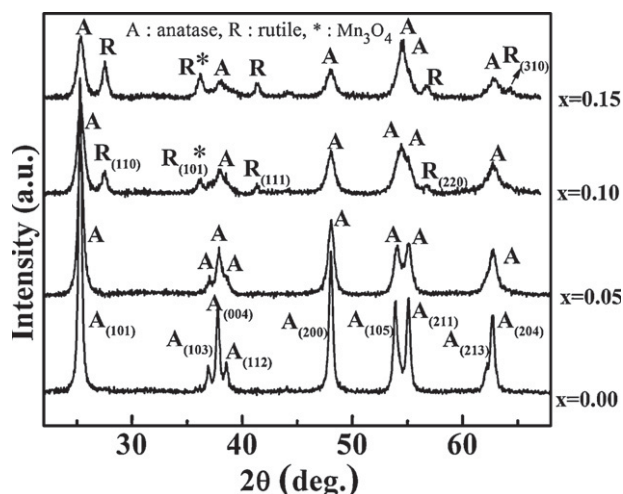
Fig. 1. X-ray diffractograms of Ti_{1-x}Mn_xO_2 nanopowders for x=0.00, 0.05, 0.10 and 0.15 .
