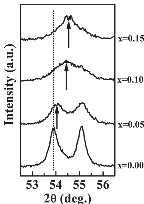
Fig. 2. Shift in (1 0 5) diffraction peak from anatase TiO_2 with the increase in Mn concentration ' x '. The arrow highlights the shift in peak position.
