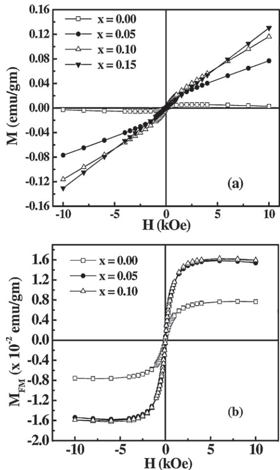
Fig. 4. M - H curves of \text{Ti}_{1-x}\text{Mn}_x\text{O}_2 nanopowders, (a) as-recorded data for x=0.00 , 0.05, 0.10 and 0.15 at 300 K, and (b) extracted M - H behavior of FM fraction for x=0.00 , 0.05 and 0.10 at 300 K.
