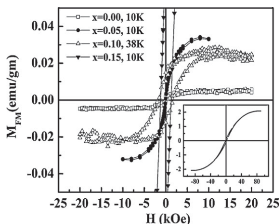
Fig. 6. Extracted M-H behavior of FM fraction of \text{Ti}_{1-x}\text{Mn}_x\text{O}_2 nanopowders for x=0.00, 0.05 , and 0.10 at indicated low temperatures. Inset shows the complete extracted M-H loop for x=0.15 sample at 10 K.
