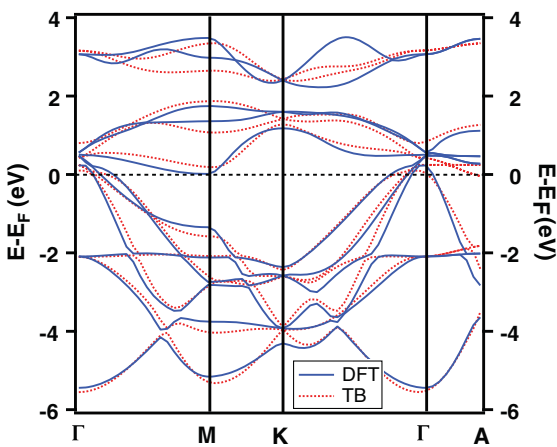
FIG. 1 (color online). Comparison of the band structure of 1T-TiSe 2 calculated with density functional theory and its fit within a TB approach.
