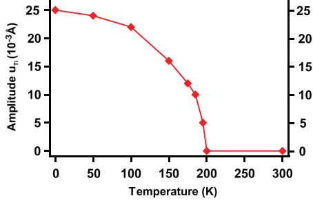
FIG. 2 (color online). Amplitude of the Ti ionic displacement for a single \vec{w}_i , u_{\text{Ti}}(\vec{w}_i, \lambda_{\text{tr}}) (the diamonds show the calculated values).
