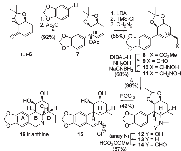
Scheme 2. Synthesis of Clivonine Progenitor 15
