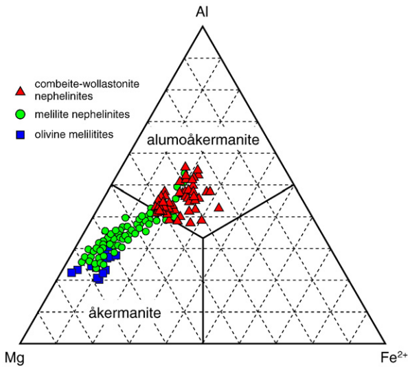
Fig. 4. Composition diagram (T1-site, at.%) of melilite from Oldoinyo Lengai in terms of åkermanite and alumoåkermanite based on the dominant-constituent rule considering Al^{3+} as the only trivalent cation on the T1-site. The data show the continuous compositional variation from åkermanite to alumoåkermanite.
