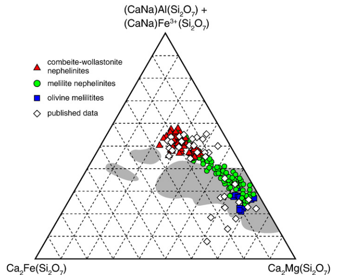
Fig. 3. Classification of Oldoinyo Lengai melilitites in terms of the components Ca_2Mg(Si_2O_7) , (CaNa)(Al,Fe^{3+})(Si_2O_7) , and Ca_2Fe(Si_2O_7) . The high sodium content of the Lengai melilitites extends the field for magmatic melilite of Velde and Yoder (1977). References for published data in the text.
