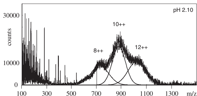
Fig. 4 ESI mass spectra of Zr solution at \text{pH}_c of 2.10. The solid lines represent Gaussian curve fitting for [i\text{-mer}]^{2+} species abbreviated to i^{++} .
