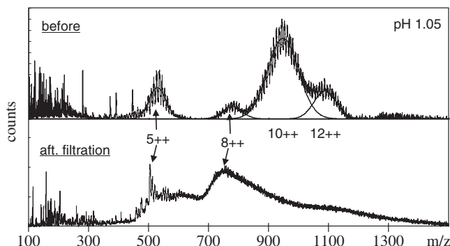
Fig. 7 Comparison of ESI mass spectra obtained before and after 3 kDa (lower) ultrafiltration. The solution is aged for 3 months at \text{pH}_c of 1.05.
