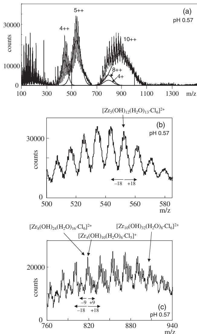
Fig. 2 ESI mass spectra of Zr solution at \text{pH}_c of 0.57. The overview spectrum (a) is shown with the solid lines of Gaussian curve fitting. The signs of i+ and i++ indicate [i\text{-mer}]^+ and [i\text{-mer}]^{2+} species, respectively. The peak clusters between m/z = 500-585 and 760-940 are magnified in (b) and (c), respectively.
