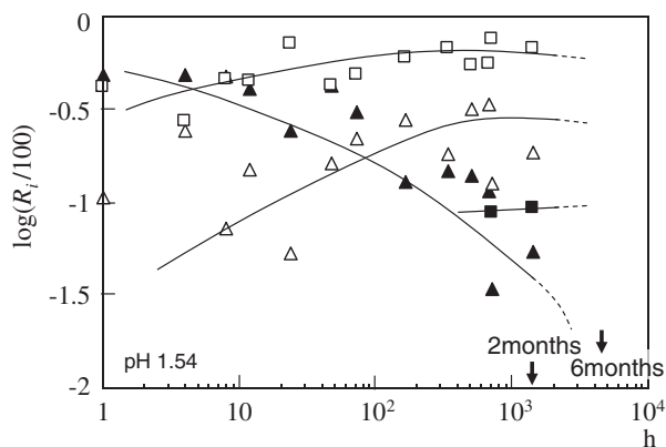
Fig. 6 Aging time dependence of polymerization in the zirconium solution at \text{pH}_c of 1.54. The symbols \blacktriangle , \triangle , \square , and \blacksquare show 5-, 8-, 10-, and 12 mer species, respectively. The error in the R_i values calculated is small relative to the plot size.
