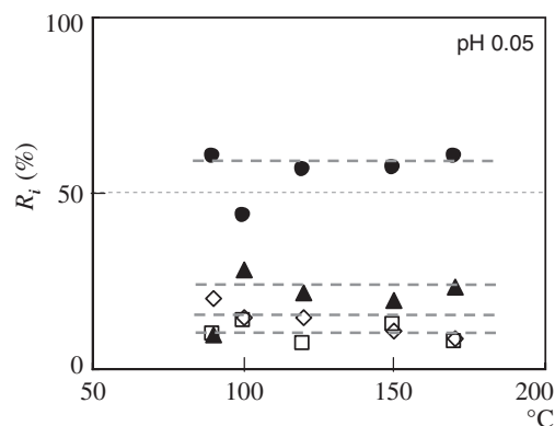
Fig. 5 Effect of the desolvation line temperature on the zirconium polymer distribution at \text{pH}_c of 0.05. The symbols \diamond , \square , \blacktriangle , and \bullet show mono-, di-, tri-, and tetramer species, respectively. The error in the R_i values calculated is small relative to the plot size.
