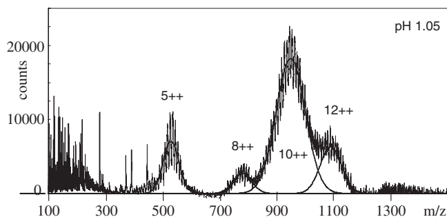
Fig. 3 ESI mass spectra of Zr solution at \text{pH}_c of 1.05. The solid lines represent Gaussian curve fitting for [i\text{-mer}]^{2+} species abbreviated to i^{++} .
