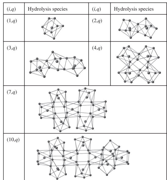
Fig. 8 Chemical structures of i -mer zirconium species assumed in the hard sphere model analysis. All hydrogen atoms in the Zr-OH-Zr bridges, hydroxyl ions, and hydrated water molecules are omitted for simple description.
