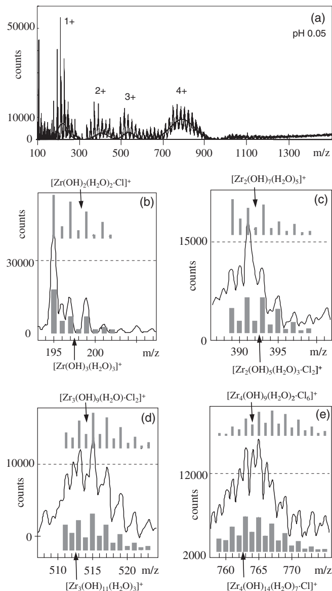
Fig. 1 ESI mass spectra in positive ion mode of Zr solution at \text{pH}_c of 0.05. The overview spectrum (a) is shown with the solid lines of Gaussian curve fitting. The signs of i+ indicate [i\text{-mer}]^+ species ( i = 1-4 ). The annotated spectra show monomer (b), dimer (c), trimer (d), and tetramer (e) species, respectively. The experimental spectra for specific complex ions are compared with the simulated isotopic patterns given in a gray bar graph. The bottom pattern for the indicated composition formula is likely assigned, while the top one is an example of the mismatches.
