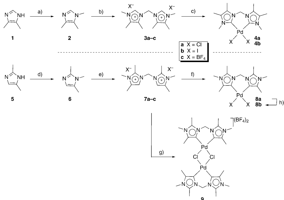
Scheme 1. a) Reagents and conditions: a) MeI, DMSO 65 °C, 18 h; b) CH 2 Cl 2 , 150 °C μwave, 0.5 h, or CH 2 I 2 , toluene 110 °C, 14 h; c) Pd(OAc) 2 , (for 3c : Pd(OAc) 2 , KCl), DMSO 120 °C, 3 h; d) Ac 2 O, benzene 80 °C, 2 h, then MeI, 140 °C, 16 h; e) CH 2 Cl 2 , μwave 150 °C, 0.5 h, or CH 2 I 2 , neat 140 °C, 16 h; f) for 7a Pd(OAc) 2 , DMSO 120 °C, 3 h; g) for 7c Pd(OAc) 2 , KCl, DMSO 120 °C, 3 h; h) AgBF 4 , MeCN, 18 h, then Bu 4 NI, MeCN 1 h.
