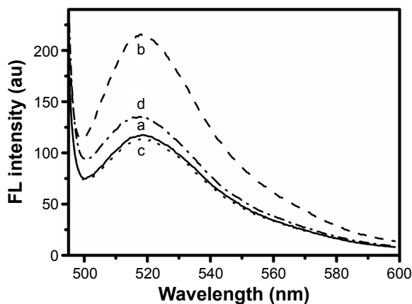
Figure 5 Fluorescence spectra of different reaction systems.
