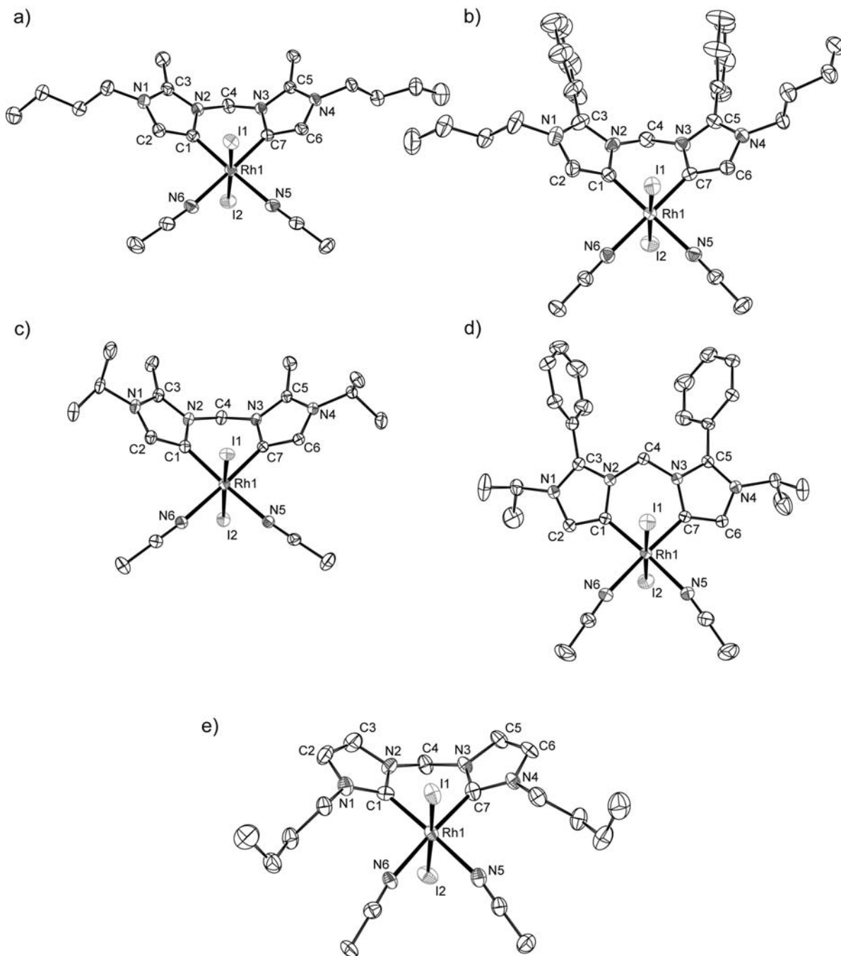
Figure 2. ORTEP representation of the cations of the C4-bound carbene complexes 3a (a), 3b (b), 3c (c), and 3d (d) and of the C2-bound dicarbene complex 3f (e). Ellipsoids are drawn at the 50% probability level ( 3c at 30%); hydrogen atoms and cocrystallized solvent molecules and I_2 (for 3c ) have been omitted for clarity.
