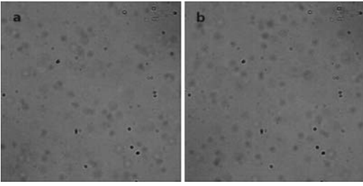
FIG. 5. Microscope images taken 10 s apart. The side of each panel corresponds to 47 \mu\text{m} in the sample. The sample is a colloidal dispersion of 420 nm particles. The more visible objects are dust particles on the CMOS sensor, which are also present in Fig. 1(a), grabbed with another sample. The particles are the less visible objects that change position between image (a) and image (b). The smearing effect due to the finite point spread function of the microscope is visible.
