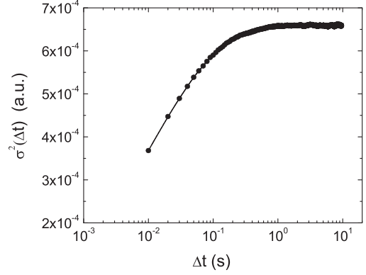
FIG. 2. The particles rearrangement due to their Brownian motion causes an increase of the variance \sigma^2(\Delta t) of the difference signal D(x, y; \Delta t) . With increasing time delay the two subtracted images become progressively uncorrelated, such that \sigma^2(\Delta t) saturates at large \Delta t .
