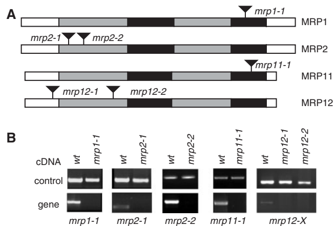
Fig. 1 Structure of the AtMRP1 , 2, 11 and 12 genes, position of insert mutants (A) and RT-PCR analysis of clade I AtMRP expression in the wild type and mutants (B). (A) Schematic structures of AtMRP1 , 2, 11 and 12 and T-DNA insertion sites. The proposed protein structure for each AtMRP is shown with two transmembrane-spanning domains (TMD1 and 2; gray bars), an N-terminal hydrophobic extension (TMD0, white N-terminal bar) and two nucleotide-binding domains (NBD1 and NBD2; black bars). The insertion sites of T-DNAs in the respective genes (filled triangles) are indicated. (B) RT-PCR analysis verifies the absence of corresponding transcripts in atmrp mutants ( mrp1-1 , mrp2-1 , mrp2-2 , mrp11-1 , mrp12-1 and mrp12-2 ) in contrast to the wild-type controls (wt). cDNAs were synthesized from total RNA of mutant and wild-type plants, and transcripts of the 40S ribosomal protein S16-encoding gene (control; upper row) were amplified and detected by RT-PCR. Furthermore, the transcripts of AtMRP1 , AtMRP2 , AtMRP11 and AtMRP12 (gene, lower row) were amplified from the cDNA of wild-type and corresponding mutant plants as indicated above each lane.
