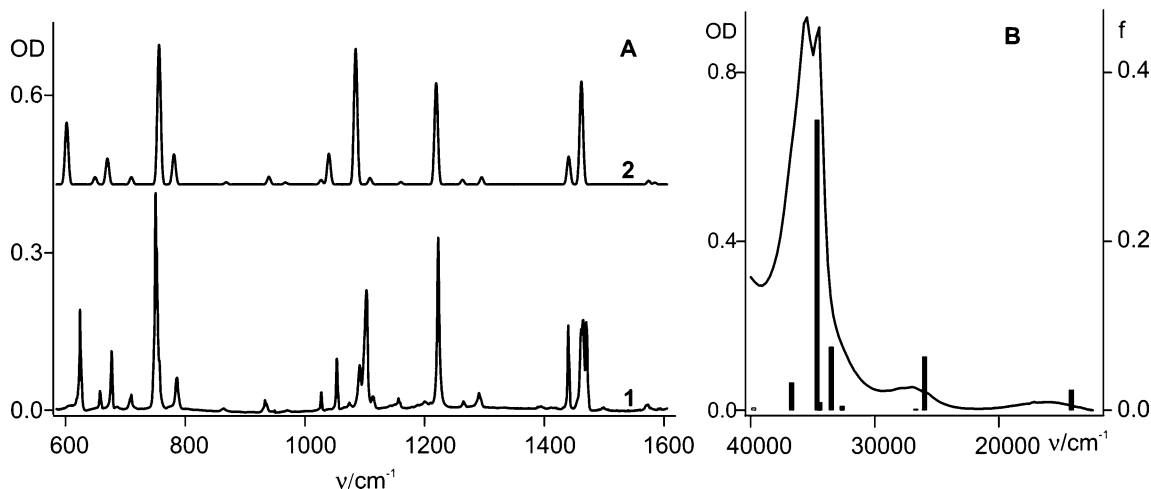
Figure 2. (A) Experimental IR spectrum of 1,3,2,4-benzodithiadiazine 1 in argon matrix at 12 K (1) and its simulation by the B3LYP/6-311G-(df,p) method with a scaling factor of 0.98 (2). (B) UV-vis spectrum of 1 in hexane at 295 K. The vertical bars indicate the positions and oscillator strengths of electronic transitions calculated by the CASSCF(16,12)/CASPT2/ANO-S method at the B3LYP/6-311G(df,p) geometry of 1 .
