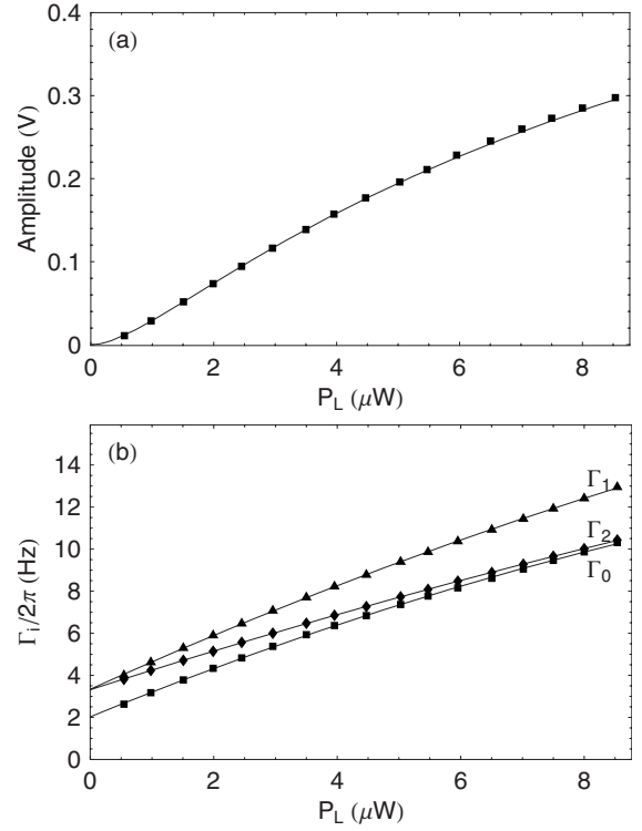
FIG. 5. (a) Second harmonic DRAM signal amplitude as a function of laser power. (b) Relaxation rates as a function of laser power. Points are measured values extracted from the fit of the DRAM model [Eqs. (3a)–(3d)] to the experimental magnetic resonance spectra. The solid lines are fits of the extended DRAM model [Eqs. (11) and (12a)–(12c)] to the experimental data. The data were measured at room temperature from a second harmonic DRAM with \gamma = 90^\circ and \omega_1 = 2\pi \times 8.3 Hz.
