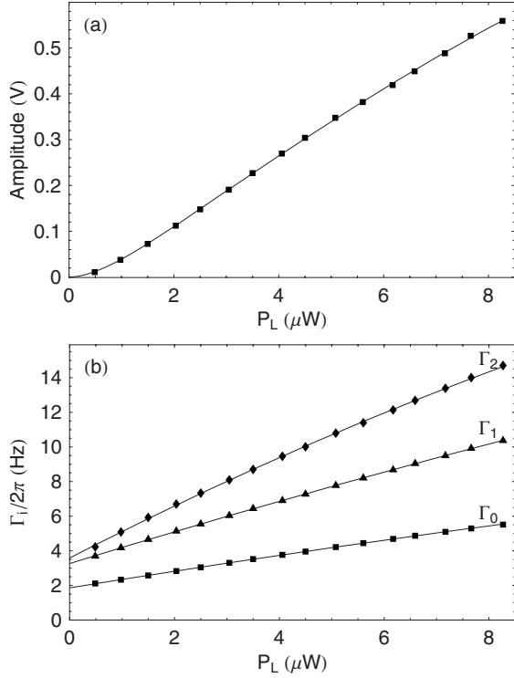
FIG. 4. (a) First harmonic DRAM signal amplitude as a function of laser power. (b) Relaxation rates as a function of laser power. Points are measured values, extracted from the fit of the DRAM model [Eqs. (3a)–(3d)] to the experimental magnetic resonance spectra. The solid lines are fits of the extended DRAM model [Eqs. (11) and (12a)–(12c)] to the experimental data. The data were measured at room temperature from a first harmonic DRAM with \gamma = 25.5^\circ and \omega_1 = 2\pi \times 8.3 Hz.
