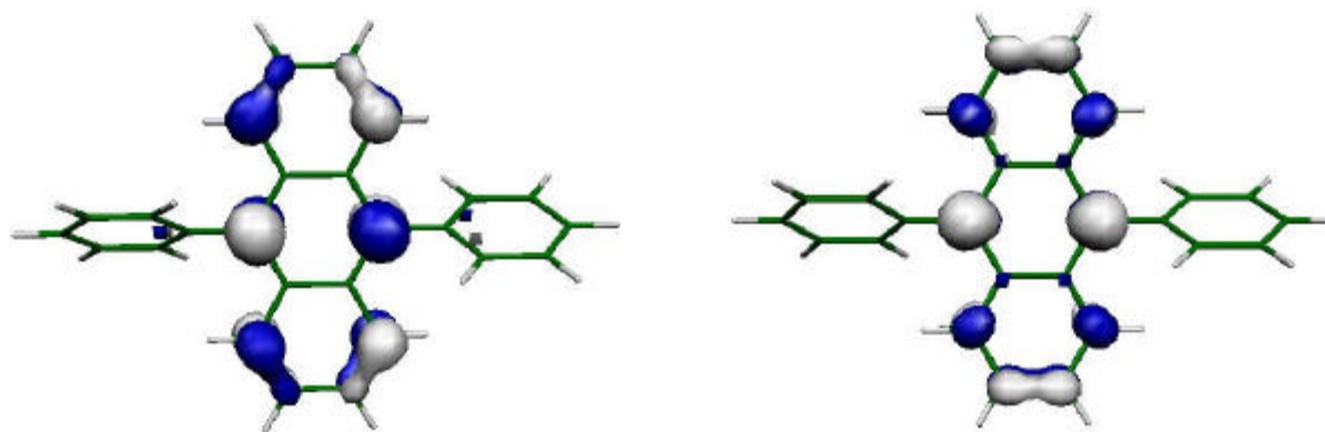
Figure SI-4. SOMOs of ^3 [ph-An-ph]. Contour value 0.05 a.u.
