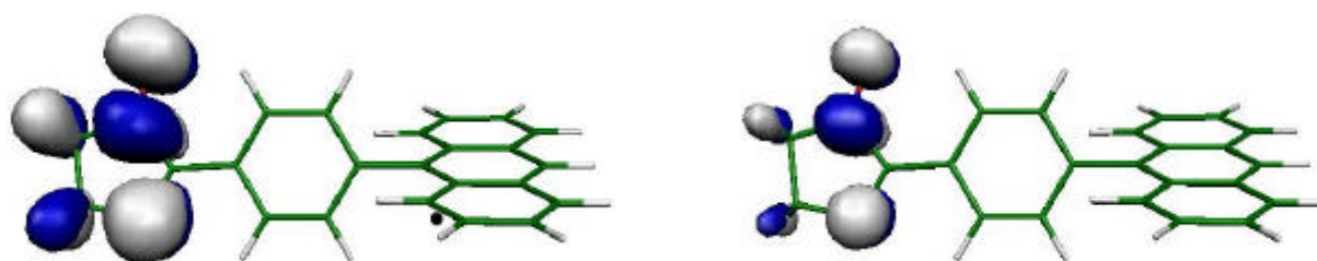
Figure SI-2. SOMO of Dd1. Contour value 0.025 a.u. (left) and 0.05 a.u. (right).
