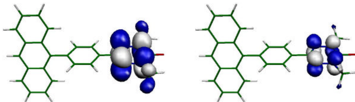
Figure SI-3. SOMO of Dd2. Contour value 0.025 a.u. (left) and 0.05 a.u. (right).
