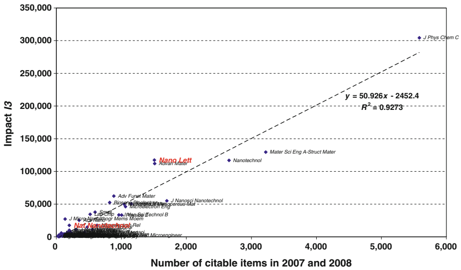
Fig. 4 Regression of impact (I3) against the number of citable publications in 2007 and 2008
