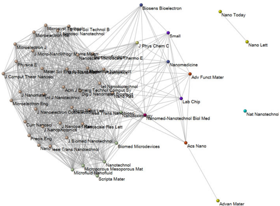
Fig. 5 Homogenous groups in terms of distribution of citation distributions among 50 journals in “Nanoscience & nanotechnology.” An edge indicates similarity in the distribution at the 5 % level ( p < 0.05/1225 ; using Bonferroni correction as explained in footnote 6)
